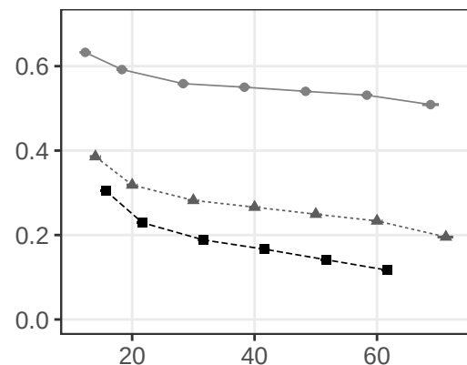
RMSE
